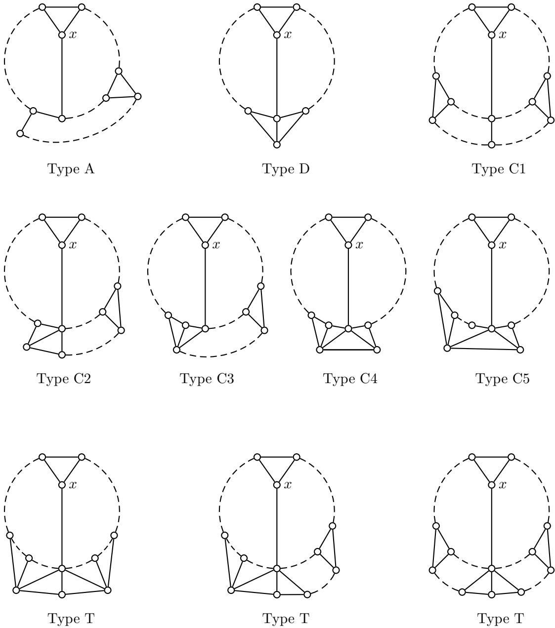
Figure 11: Bridges of a bug (H, x) .
