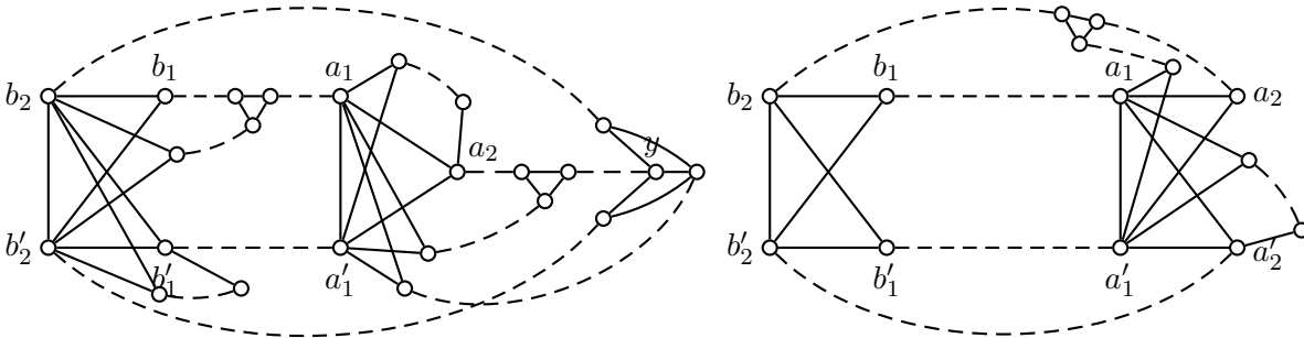
Figure 17: Paths from Lemma 9.5.
