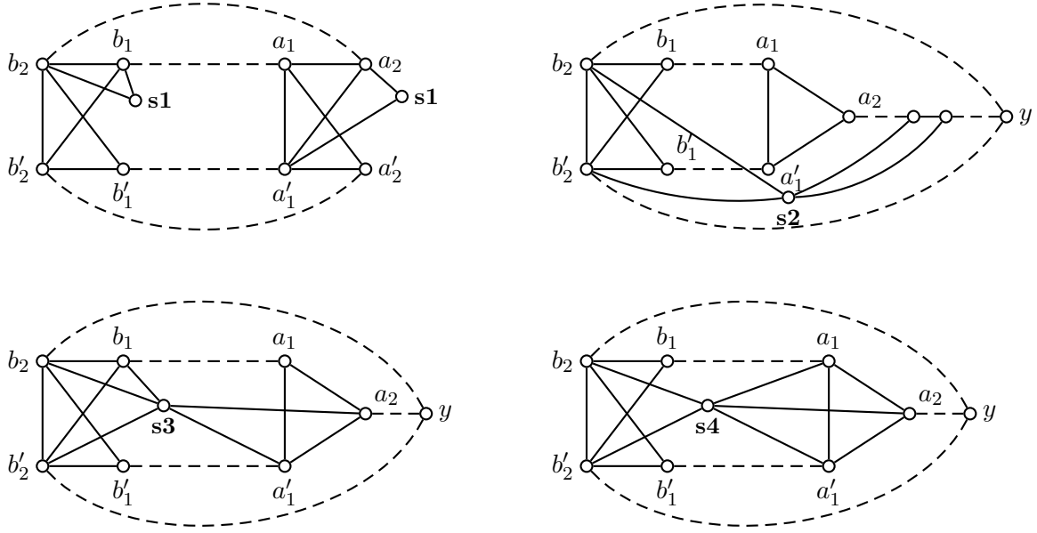
Figure 16: Nodes adjacent to a connected diamond that lead to star cutsets.
