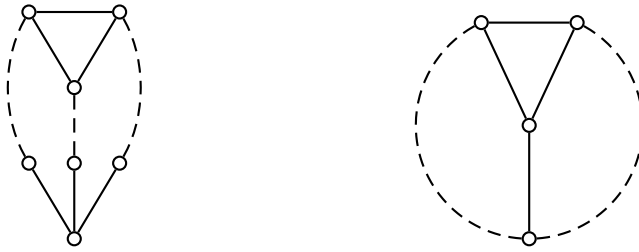
Figure 2: A long 3PC(\Delta, \cdot) and a bug.
