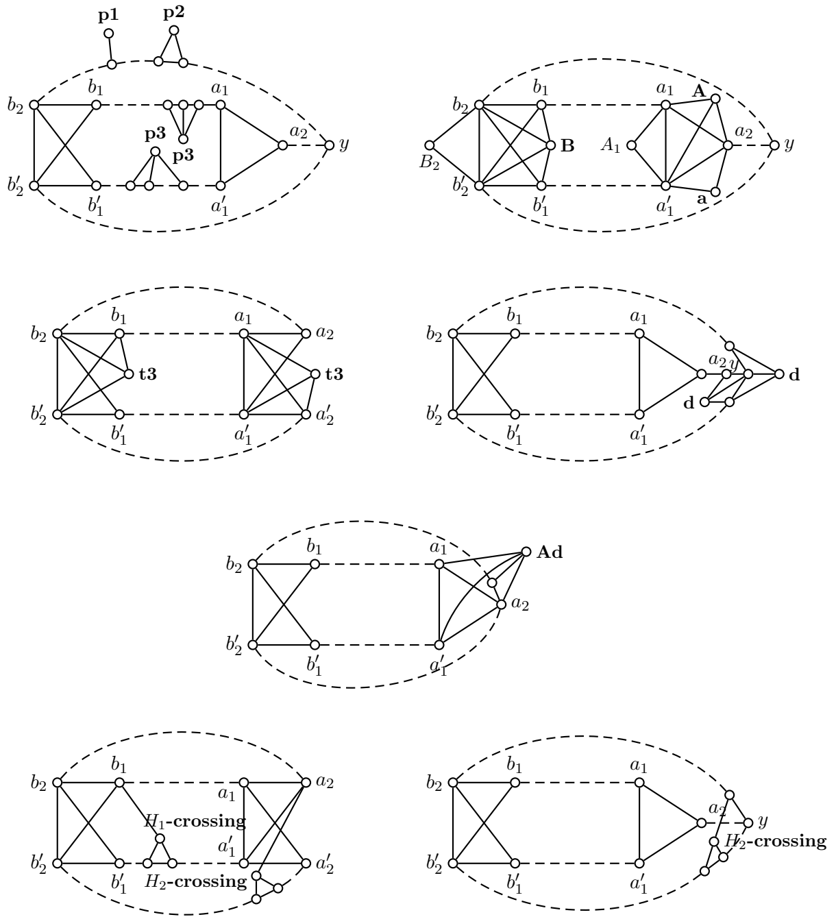
Figure 13: Nodes adjacent to a connected diamond.
