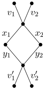
Fig. 7: Root graph of the gadget depicted in figure 6
