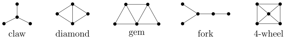
Fig. 1: Claw, diamond, gem, fork and 4-wheel
