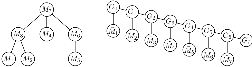
Fig. 9: A standard modular decomposition tree and its extended tree
